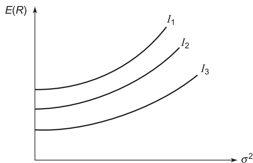
Exhibit 22.2 Indifference Curves
