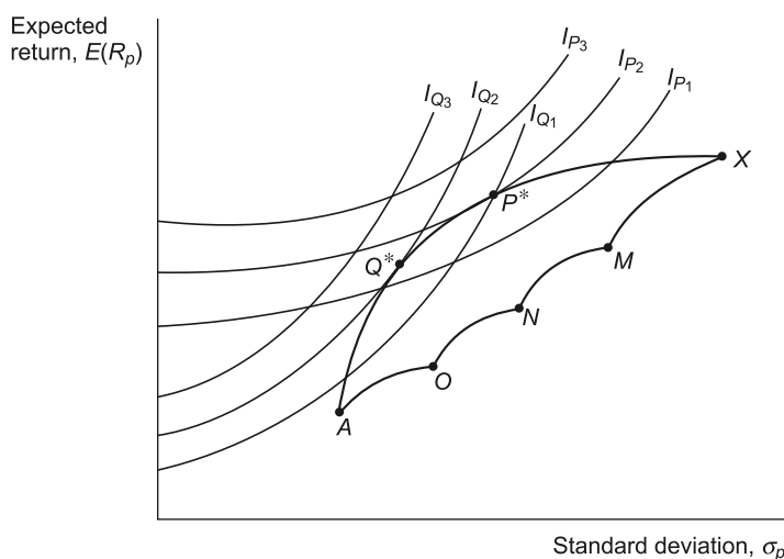
Exhibit 7.13 Optimal Portfolio
