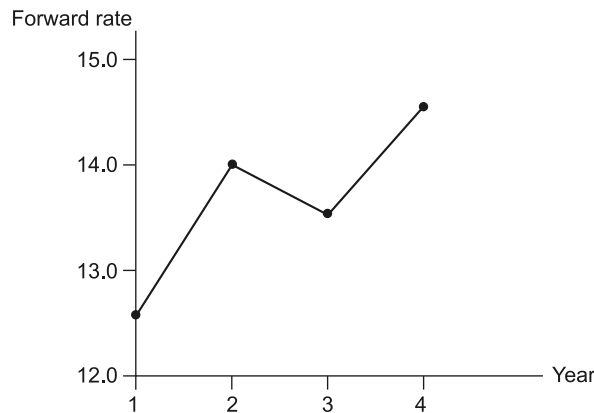
Exhibit 11.7 Forward Rates
