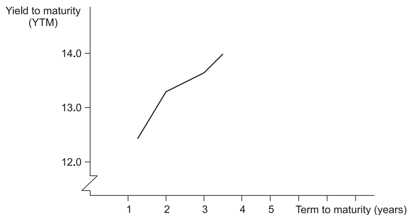
Exhibit 11.5 Yield Curve
