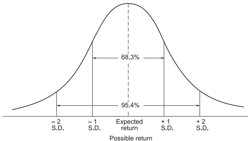
Exhibit 4.5 Normal Distribution
