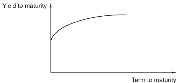
Exhibit 11.8 Yield Curve
