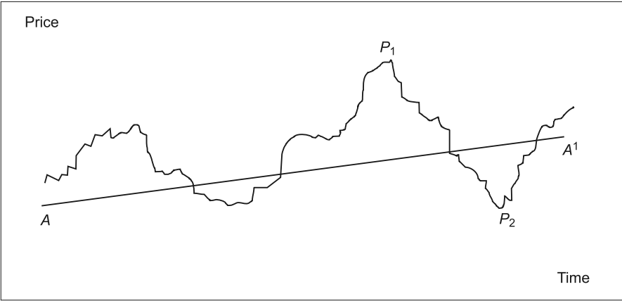
Exhibit 25.4 Price Behaviour
