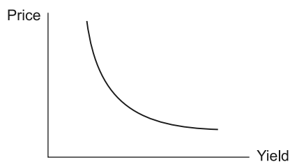
Exhibit 11.2 Price-Yield Relationship
