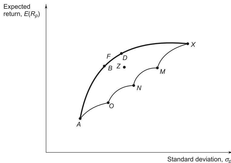
Exhibit 7.9 Feasible Region
