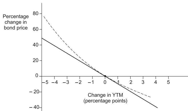
Exhibit 12.4 Bond-Price Convexity
